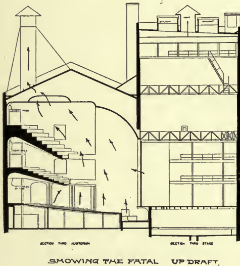
SHOWING THE FATAL UP DRAFT.
